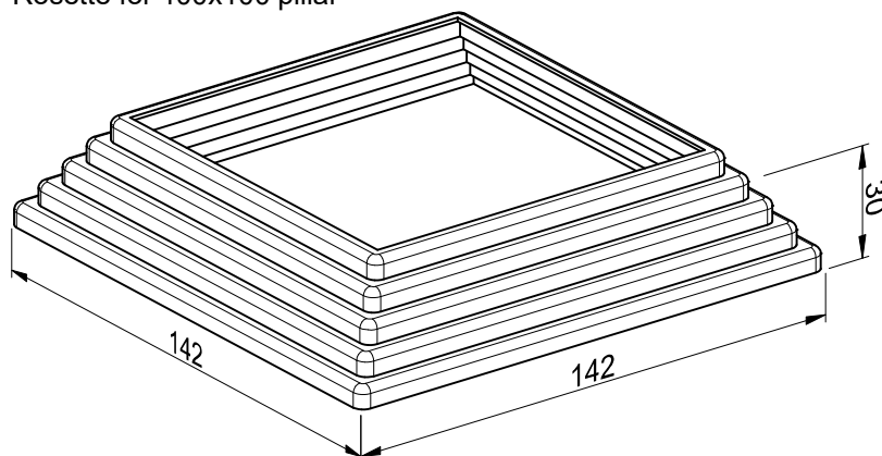
F25 Rozeta stuba 100x100 Rosette for 100x100 pillar
