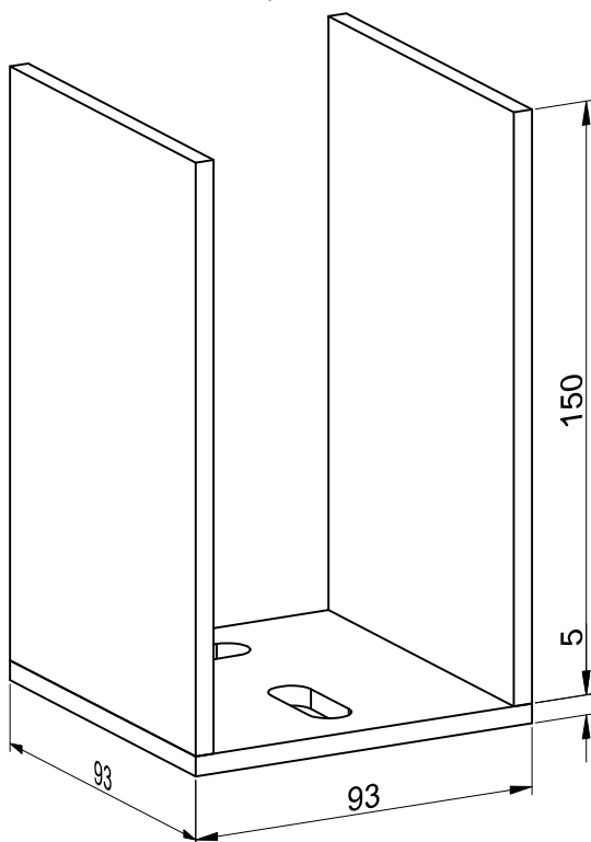
F17 Kotva stuba 100x100 Anchor for 100x100 pillar
