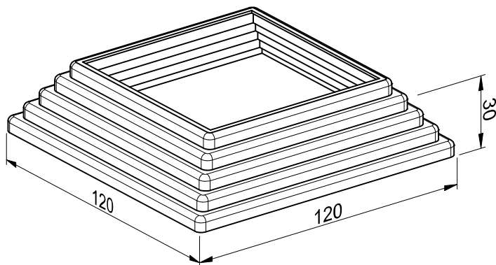
F25 Rozeta stuba 100x100 Rosette for 100x100 pillar
