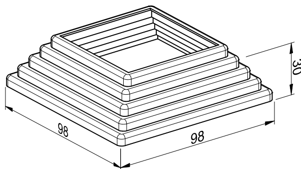
F23 Rozeta stuba 60x60 Rosette for 60x60 pillar
