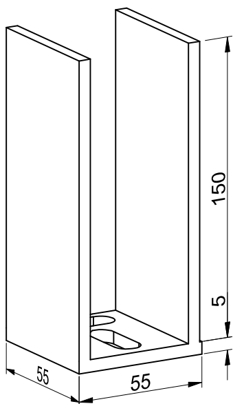
F16 Kotva stuba 60x60 Anchor for 60x60 pillar
