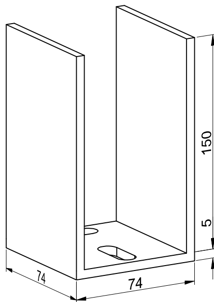
F15 Kotva stuba 80x80 Anchor for 80x80 pillar
